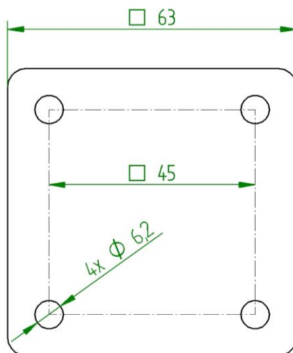
Luminaire mounting drawing:
