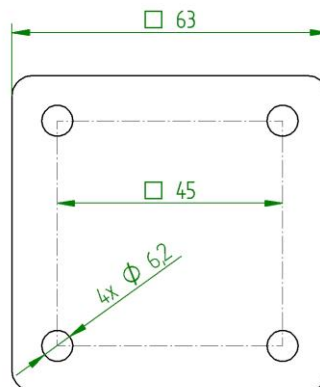
Luminaire mounting drawing:
